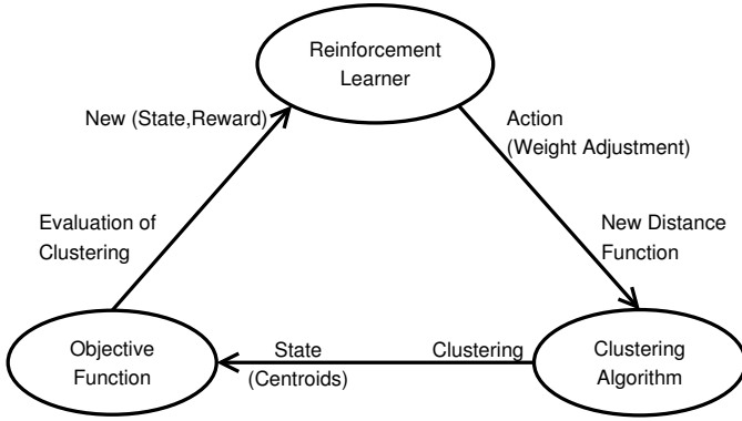
Fig. 1. The adaptive clustering environment.
