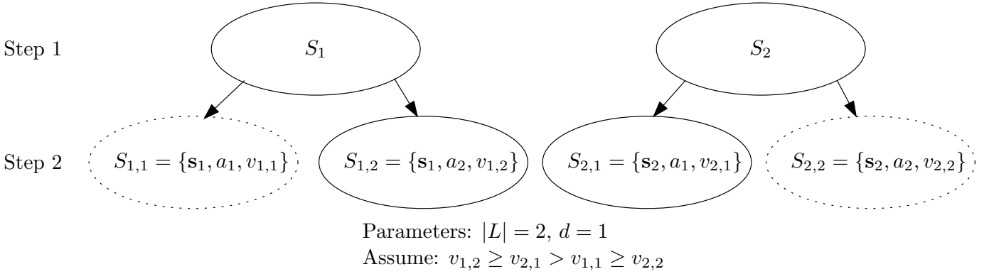
Fig. 2. The adaptive clustering search strategy.
