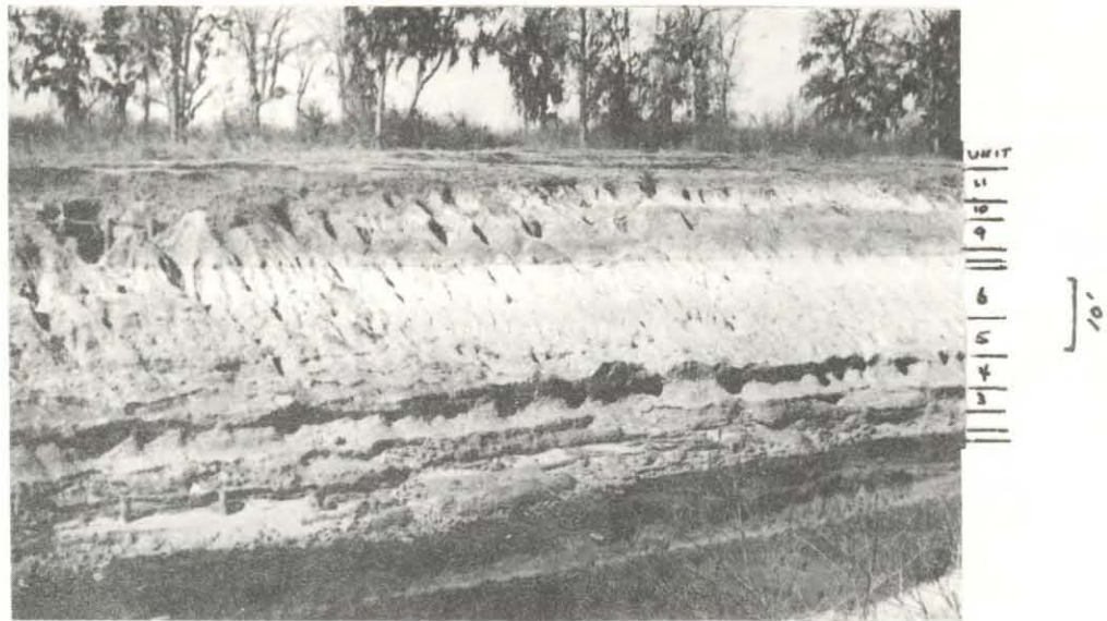
Figure 10. Layers of sand and clay exposed along White Oak Bayou, 50 yards downstream (southeast) from the 18th Street bridge in Houston. The darker material in the upper third of the bank is clay (mostly red), the light material along the central part of the bank is sand (white to gray and brown), and below that the material is mostly clay again, with three to four feet of somewhat consolidated sand near the middle of it. Height of the exposure is 33.2 feet. (From Gordon A. Clopine 1960.)
