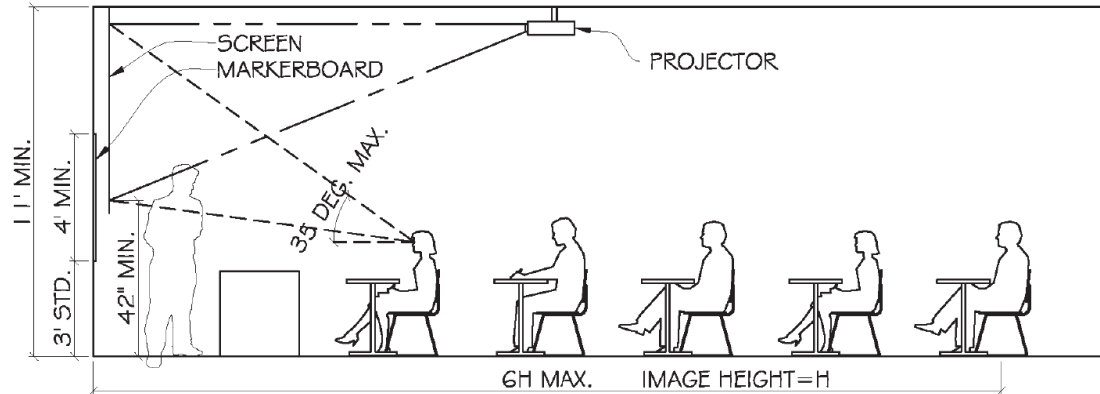
FIGURE 3: TIERED-FLOOR ROOM SECTION WITH RETRACTABLE SCREEN, WITH STANDARD MEASUREMENTS
