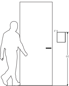
Mounting Guidelines (Wall-Stairwell Side) Sign to mount with VHB foam tape and silicone
