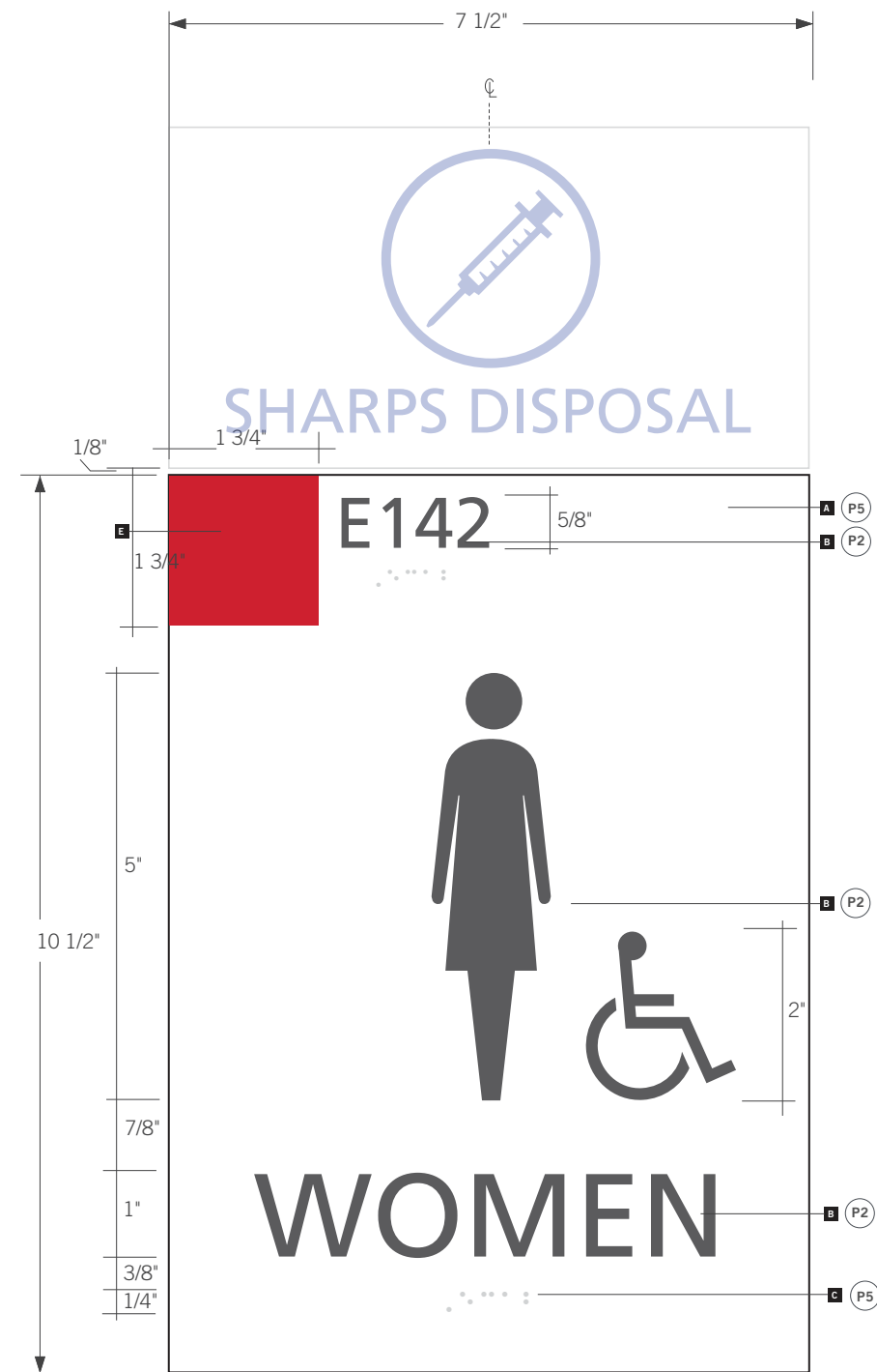
Layout (TYPICAL MEN AND WOMEN)
