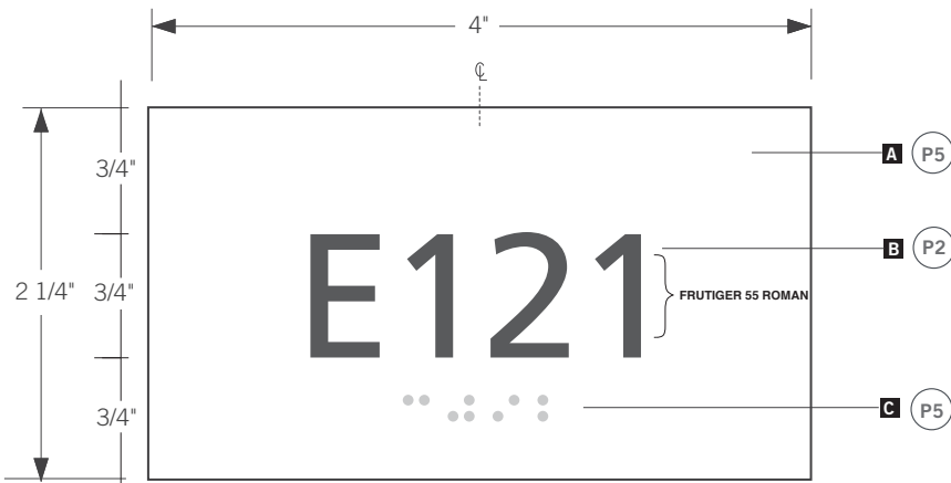
Type C, Numbering Plaque
