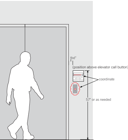
Mounting Guidelines (wall) Sign to mount with VHB foam tape and silicone
