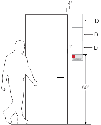
Mounting Guidelines (wall - Hallway side) As single holders or in multiples Sign to mount with VHB foam tape and silicone
