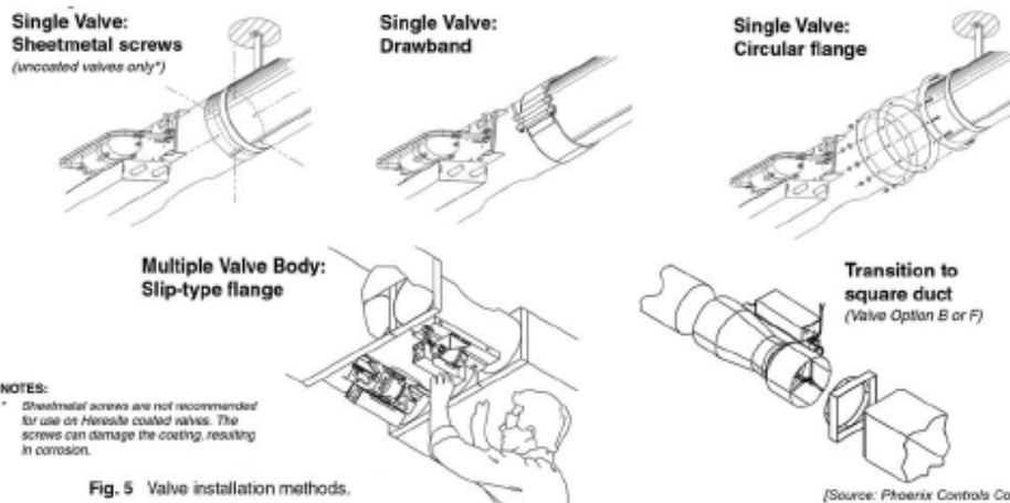
Fig. 5 Valve installation methods.
