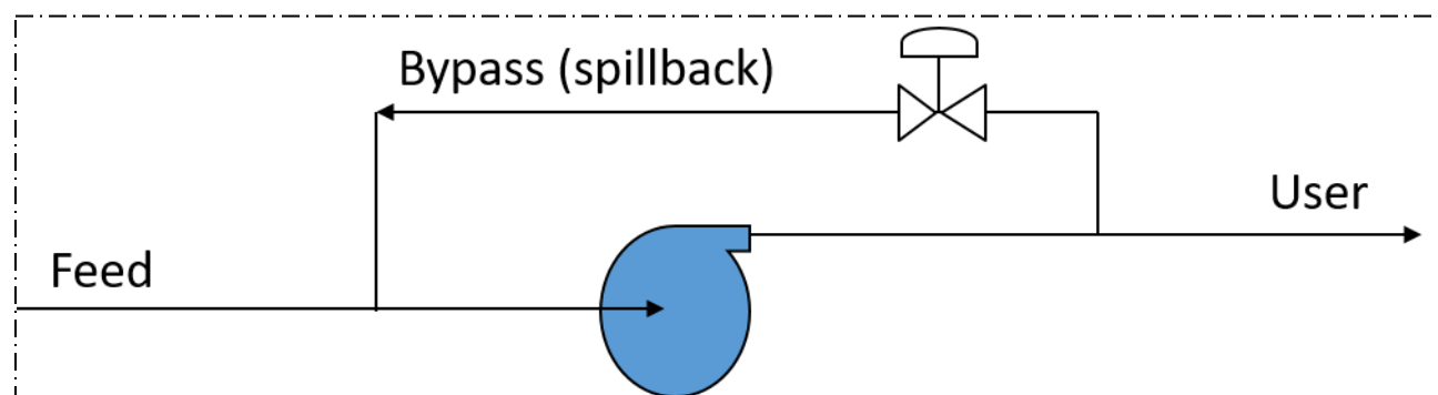
Figure 1: Bypass Control
