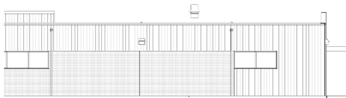
② North elevation 3/2" = 1'-0"
