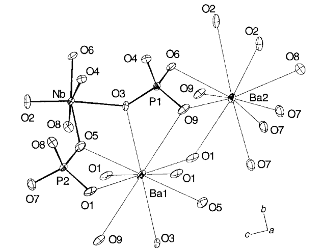
Fig. 1 Local coordination of cations in Ba 3 (NbO) 2 (PO 4 ) 4 . Thermal ellipsoids are at 50% probability.
